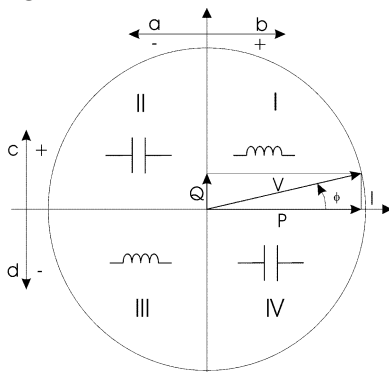
Fig. 2 : Geometric Representation
